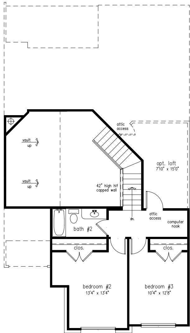
Second Floor
